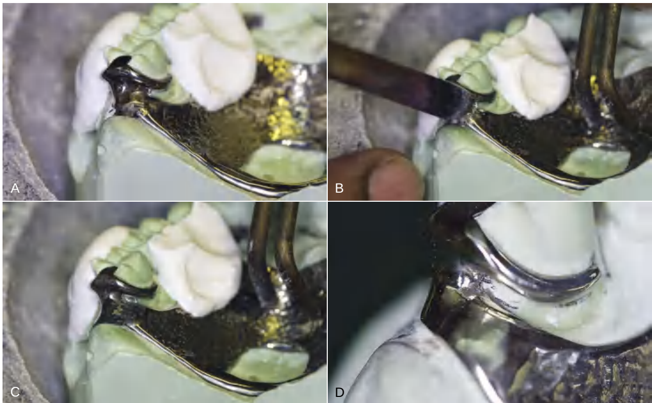
FIGURE 22-2 A , The maxillary junction between major and minor connectors at the distalmost posterior molar has fractured. Thin platinum foil has been adapted to the cast beneath the fracture, the clasp assembly has been stabilized on the cast with fast-set plaster, the remainder of the prosthesis has been positioned on the cast in full contact with teeth and tissues, and the solder has been positioned for the electric tip to be placed. B , The electric soldering tip and ground are in place. C , Immediately following solder flow, the fracture has been eliminated by the solder connecting the two segments. D , The polished solder repair is ready to be cleaned and returned to the patient. The patient is told that this repair is not as strong as the original, and although it is difficult to know how long it could serve the patient, careful handling of the prosthesis is mandatory.
