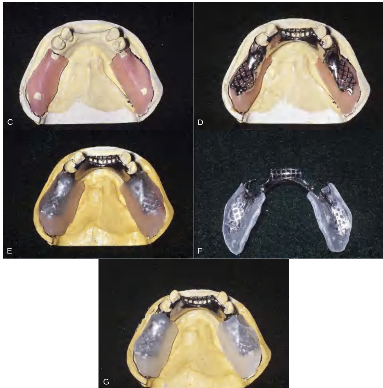
FIGURE 16-8, CONT'D C , One thickness of baseplate wax is adapted to outlines to act as spacers so that room for the impression material exists in the finished trays. Windows are cut in the wax spacers corresponding to regions on the cast contacted by minor connectors (tissue stops) for denture bases. D , The framework is warmed and pressed to position on the relieved master cast. All regions of the cast that will be contacted by autopolymerizing acrylic-resin or visible light-cured (VLC) resin are painted with tinfoil substitute (Alcote) or model release agent (MRA). E , Acrylic-resin material is adapted to the cast and over the framework with finger pressure as described in Chapter 15. Excess material over the borders of the cast is removed with a sharp knife while the material is still soft. F , Polymerized acrylic-resin trays and framework are removed from the cast, and trays are trimmed to outline the wax spacer. G , Borders of the trays will be adjusted to extend 2 mm short of the tissue reflections. Holes will be placed in the trays corresponding to the crest of the residual ridge and retromolar pads to allow escape of excess impression material when an impression is made.
