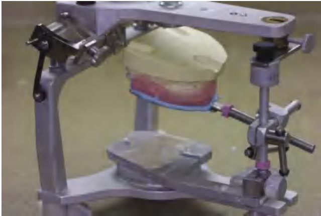
FIGURE 12-10 Facebow fork support used to maintain the fork and cast in position while mounting.
