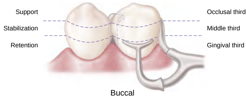
FIGURE 7-20 Only one terminal of the retentive arm engages the undercut in the gingival third of the abutment. The suprabelge portion of the retentive clasp arm provides only limited stabilization and may be eliminated.
