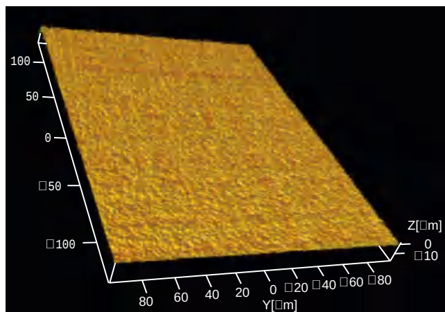
Figure 16-3 Implants manufactured from titanium alloy, which represents a hard material, may demonstrate a very smooth surface outcome if a similar manufacturing approach, such as with softer CP titanium, is applied. Nano Tite PREVAIL implant with an Sa of 0.3 \mu\text{m} and an Sdr% of 17.
