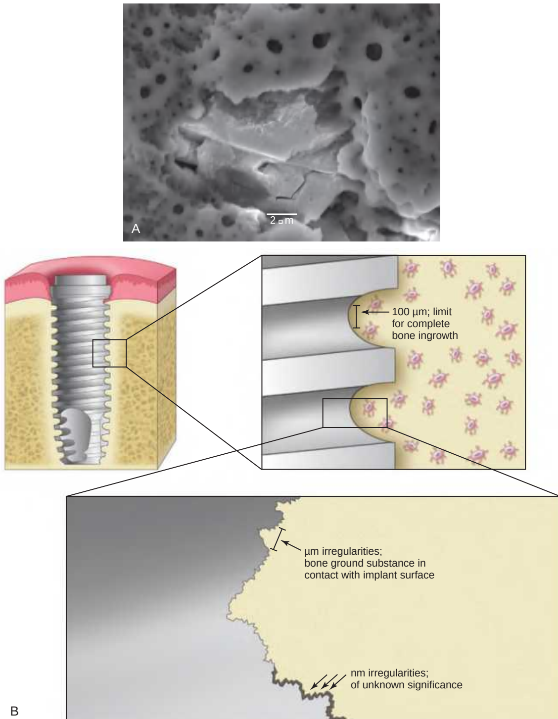
Figure 16-1 A , A moderately rough surface characterized by an Sa of 1 to 2 μm and an Sdr% of 25 to 75 may serve as an example of most commercially available modern implants. This image presents a moderately rough blasted and anodized surface, with typical porosity achieved by anodisation. B , Bone tissue including ground substance and cellular components will need pores of a minimal size of 100 μm for ingrowth. Calcified ground substance of bone responds differently to irregularities in the micrometer size that are important for the strength of the osseointegrated response. Implant irregularities in the micrometer range are, to date, of undetermined significance for osseointegration.
