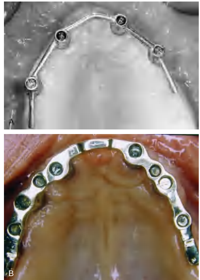
Figure 17-6 A, The maxilla's ridge contour is reflected in a segmented bar soldered to four implant abutments. B, Rigid splinting of multiple implants using a cast milled bar. Retentive clips or attachments can engage any or all of the available segments, ensuring good retention, optimal prosthetic teeth placement, and nonrestriction of tongue space.
