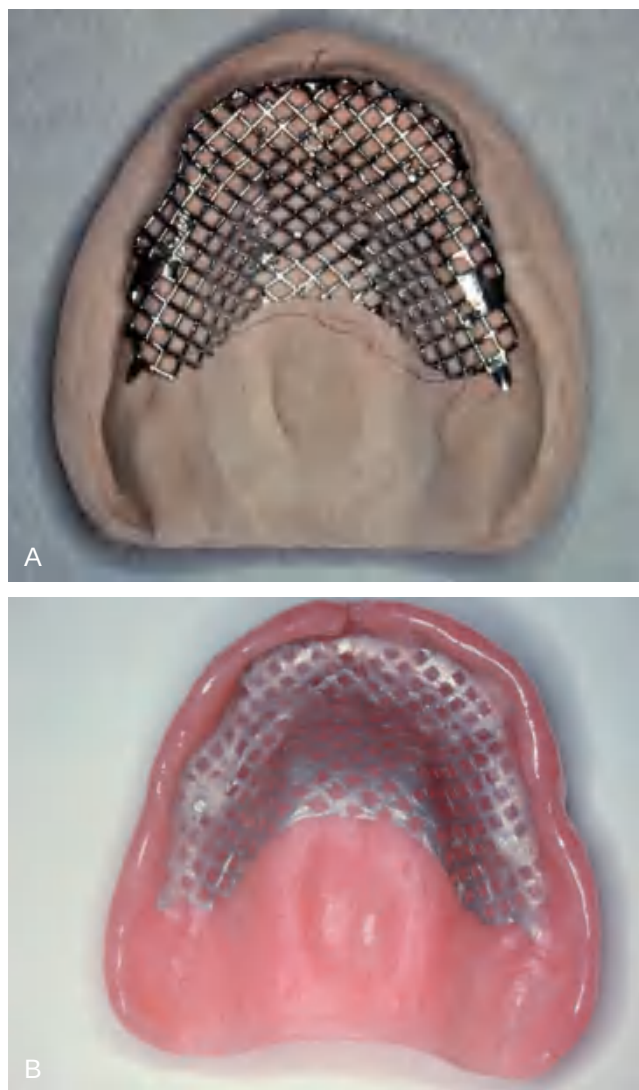
Figure 13-18 A , Plan on cast Cr-Co mesh reinforcement if intact arch and heavy function. B , Cast mesh is embedded in PMMA at processing.
