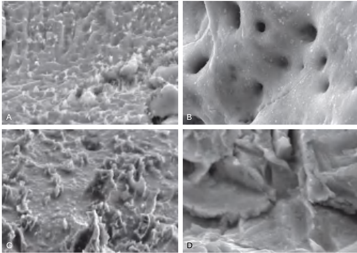
Figure 16-4 Modern implants display clear nanopatterns in contrast to their respective predecessors. A , Astra Tech OsseoSpeed implant. B , Nobel BiocareTiUnite implant. C , A Biomet 3i Nanotite implant. D , An example of a predecessor implant Astra TiOblast without the typical nanopattern. All images 50,000x or more in magnification.
