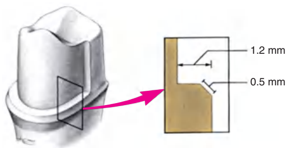
Fig. 9-17 The shoulder bevel.
