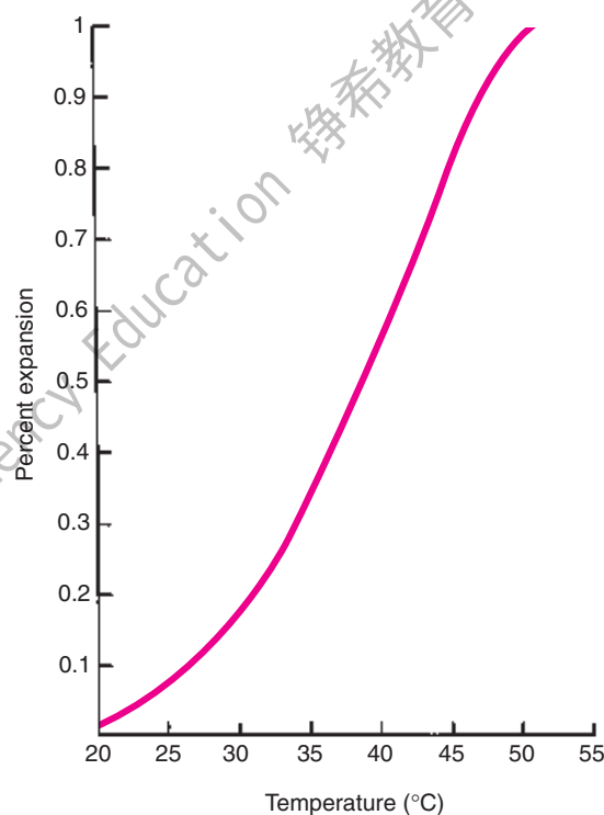
Fig. 18-7 Wax expansion curve.
