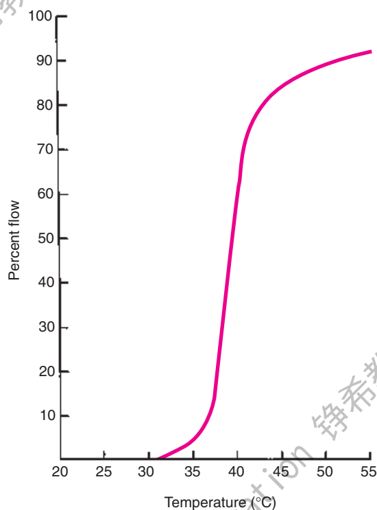
Fig. 18-6 Wax flow curve.
