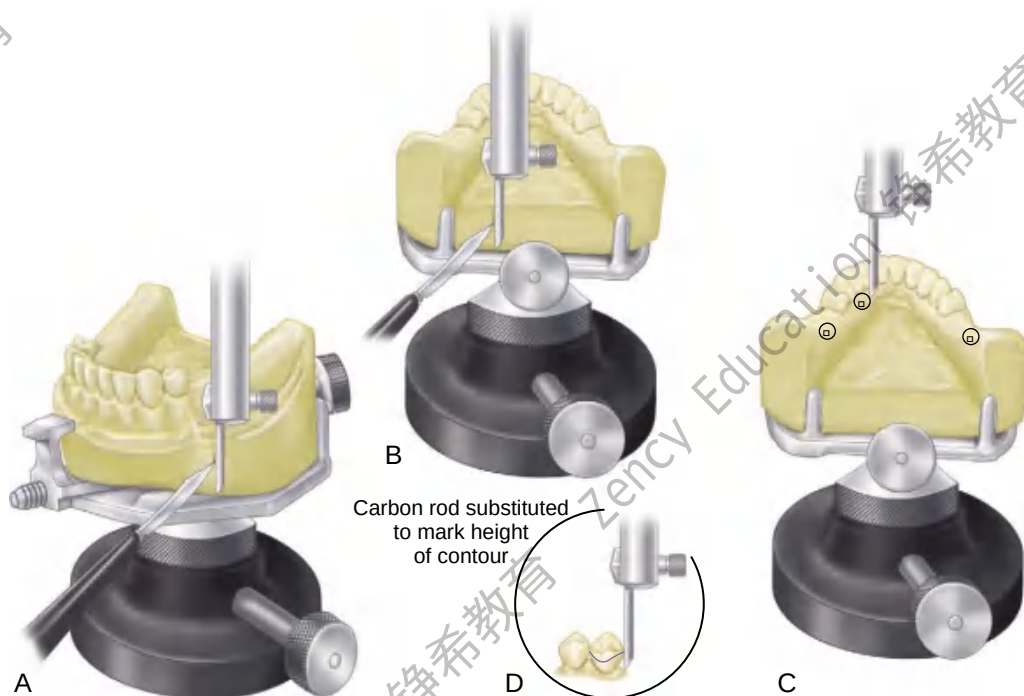
FIGURE 11-15 A-B , The path of placement is determined, and the base of the cast is scored to record its relation to the surveyor for future repositioning. C , An alternate method of recording the relation of the cast to the surveyor is known as tripoding . A carbon marker is placed in the vertical arm of the surveyor, and the arm is adjusted to the height by which the cast can be contacted in three divergent locations. The vertical arm is locked in position, and the cast is brought into contact with the tip of the carbon marker. Three resultant marks are encircled with colored lead pencil for ease of identification. Reorientation of the cast to the surveyor is accomplished by tilting the cast until the plane created by three marks is at a right angle to the vertical arm of the surveyor. D , Height of contour is then delineated by a carbon marker.
