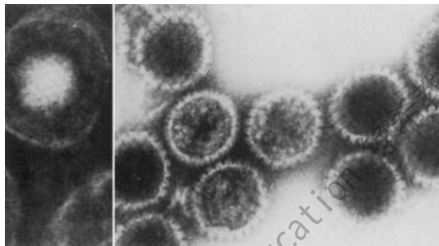
Fig. 8.26 Herpes simplex virus type 1. Electron micrographic picture of herpes simplex virus type 1, enveloped (left) and naked capsids (right). \times 198,000 . (From Fields BN, Knipe DM: In Fields BN, editors: Virology, New York, 1985, Raven Press.)
