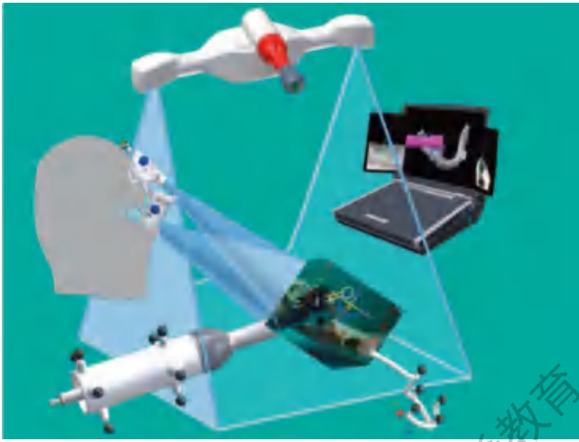
Fig. 84.3 Global setup for surgical navigation. The basic setup for a navigation system consists of stereovision cameras with several tools. The contra-angle probe, the ultrasound probe, and the patient jig need to have markers, which are tracked by the cameras. The occlusal stent, with markers in the standard process and without markers in ultrasound registration, used during computed tomography scan acquisition will be recognized in its three dimensions for prosthetic planning.
