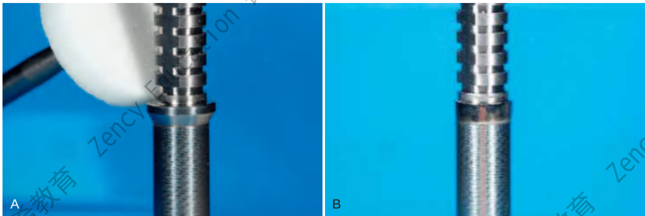
eFig. 77.7 Temporary abutments from some manufacturers have a flared area that comes directly off the head of the implant. This is a flawed design and the flared area should be removed prior to use with a heatless stone (A). Once removed, the area should be no wider than the implant and must be polished (B).
