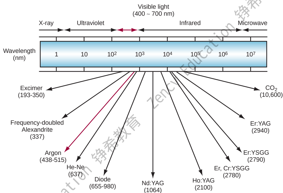
Fig. 68.3 Laser wavelengths. Each laser has a unique wavelength spectrum resulting in specific absorption characteristics. The wavelength of most of the lasers used in dentistry/periodontics is in the red and near-infrared spectrum.
