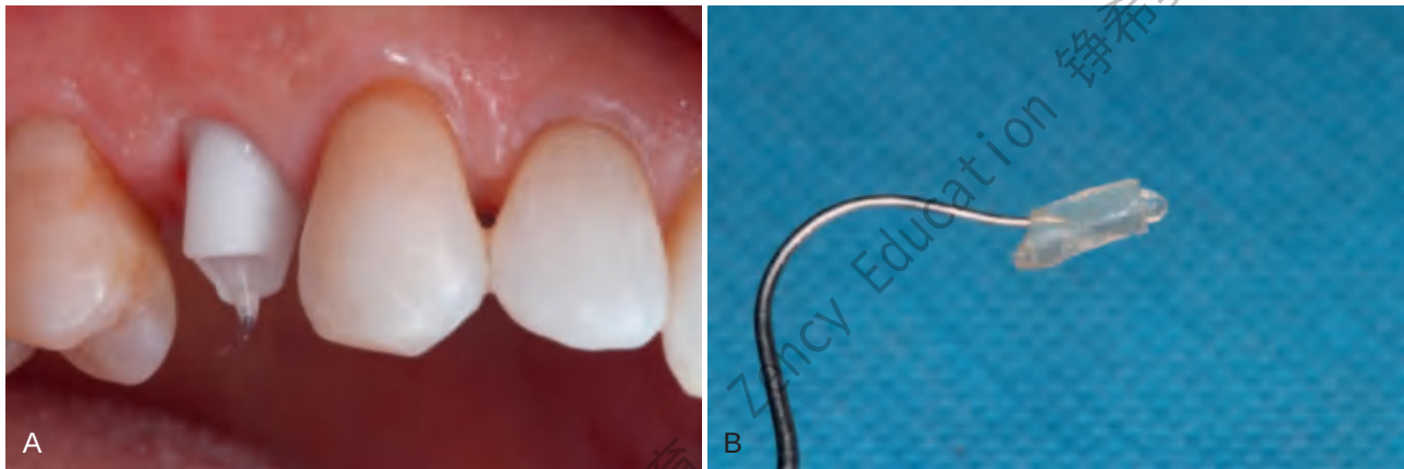
eFig. 77.3 PVS impression material also works well to cover the abutment screw, though it is best suited for use with cemented restorations. The material is dispensed into the screw access starting at the bottom and back-filling to the top (A). The excess is then wiped off before setting and cementation of the crown. The PVS plus is easy to remove should the need arise (B).
