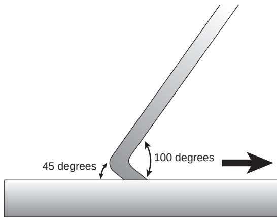
eFig. 50.74 Back-action chisels and hoes are sharpened with a pull stroke.
