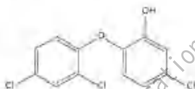
Figure 16.5 The molecular formula of triclosan.
