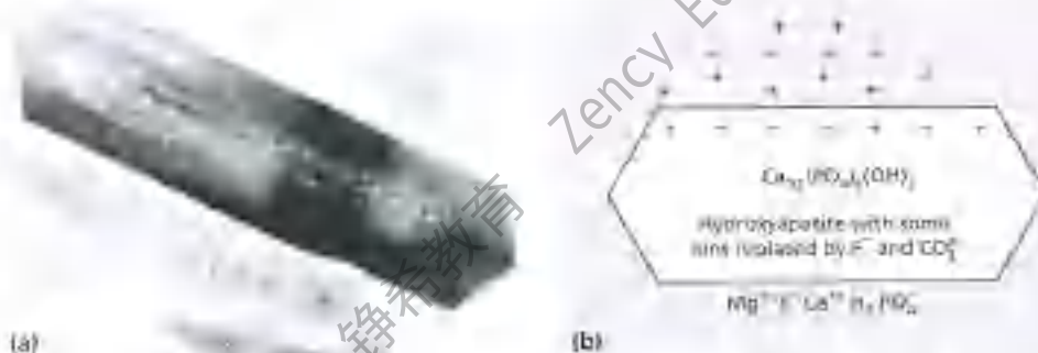
Figure 9.1 (a) Cross-cut enamel crystal from a heavily mineralized human enamel. The hexagonal crystal exhibits a dark central line and a lattice striation with an interval of 0.617 nm (–0.2 Å) between the lines which intersect each other at an angle of 60° reflecting the unit cell of hydroxyapatite. (b) Reproduced with permission of Oxford University Press. (b) Schematic drawing of a ‘typical’ enamel crystal. These crystals are about 350 Å in thickness and 1200 Å in width. Ions in the hydration shell can easily be exchanged. Some ions are bound in the hydroxyapatite lattice (e.g., fluorine is not easily exchanged unless the crystal is dissolved). For an explanation of the drawing, please see the text.
