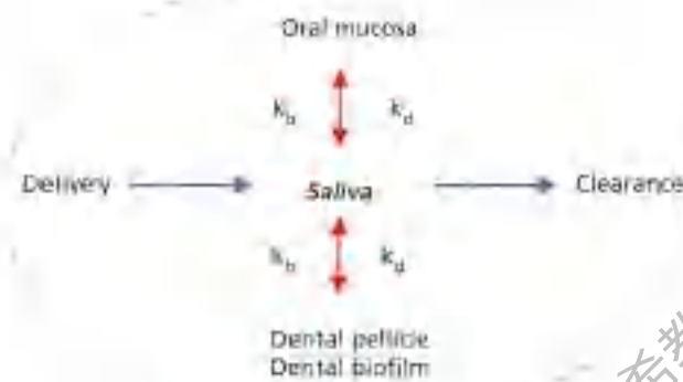
Figure 16.1 Oral delivery, binding, release, and clearance of antibacterial agents in the oral cavity. The agent binds to oral mucosa, tooth surfaces, pellicle, and dental biofilm bacteria according to its affinity k_b and released from its binding site depending on its dissociation constant k_d and salivary clearance rate. The oral mucosa represents the major reservoir for substantive agents. After [50]. Reproduced with permission of Sage Publications.
